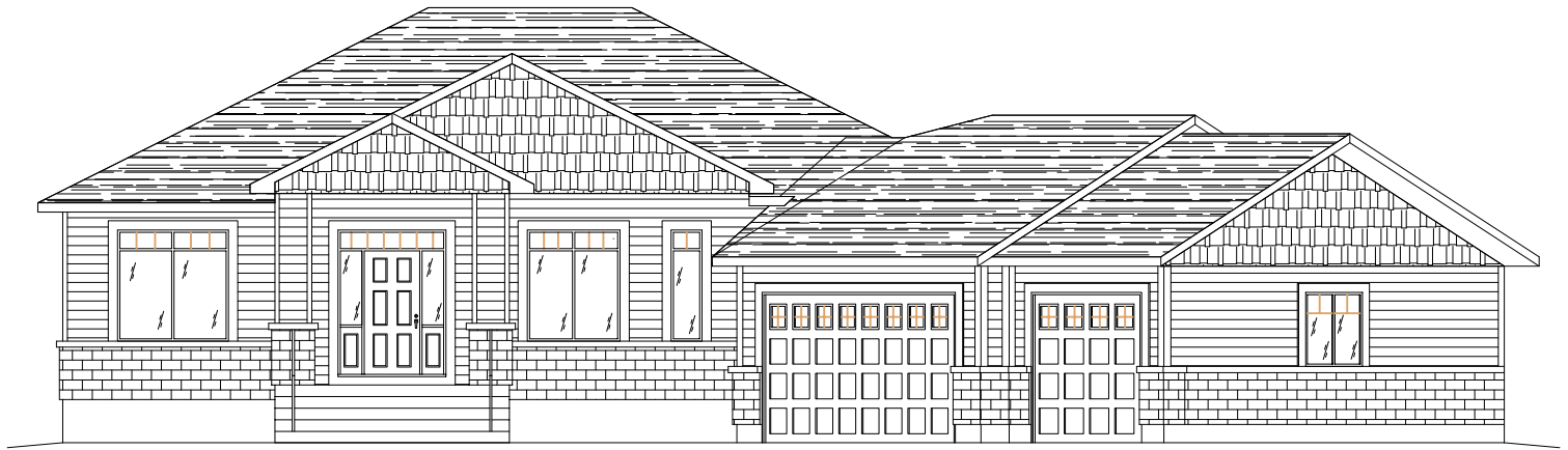
-FRONT ELEVATION-
